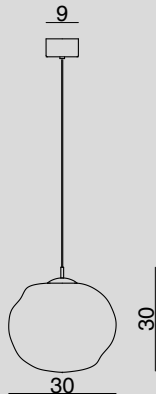
GIG1643.1L SOSPENSIONE A ROSONE / HANGING LAMP WITH CANOPY Glass 1 x Ø 30 cm - Cable 200 cm 1 x LED 8,4 W DIMM
