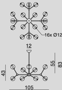
1574.12.4.16L LAMPADARIO / CHANDELIER Glass 16 x Ø 12 cm 16 x G9 33 W
