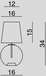
LU1203 LAMPADA DA TAVOLO / TABLE LAMP Glass 1 x Ø 16 cm - Cable 200 cm 1 x E14 40 W
