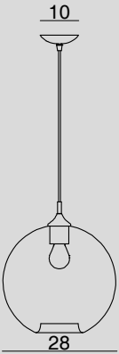
GIG1203.1L SOSPENSIONE A ROSONE / HANGING LAMP WITH CANOPY Glass 1 x Ø 28 - cmCable 150 cm 1 x E27 70 W
