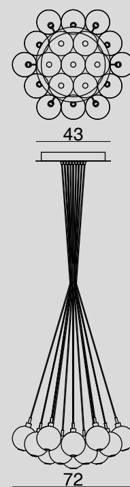
1292.19L SOSPENSIONE A PIASTRA / HANGING LAMP WITH CEILING PLATE Glass 19 x Ø 14 cm - Cable 250 cm 19 x G9 33 W
