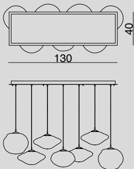
1679MX.40X130.7L SOSPENSIONE A PIASTRA / HANGING LAMP WITH CEILING PLATE Glass 7 x Ø 30-30-35 cm - Cable 200 cm 7 x LED 8,4 W DIMM
