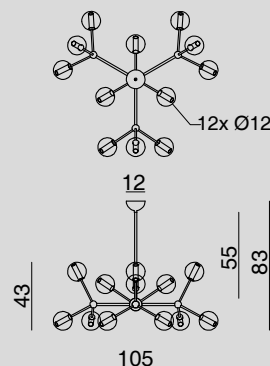
1574.9.3.12L LAMPADARIO / CHANDELIER Glass 12 x Ø 12 cm 12 x G9 33 W
