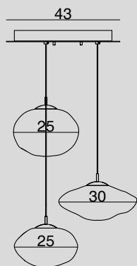
1679MX.43.3L SOSPENSIONE A PIASTRA / HANGING LAMP WITH CEILING PLATE Glass 3 x Ø 25 - 30 - 25 cm - Cable 200 cm 3 x LED 6 W DIMM
