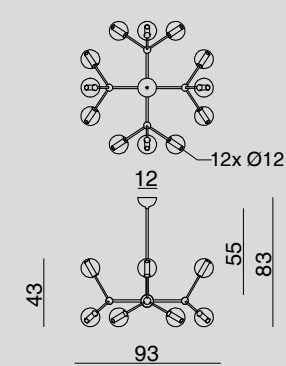
1574.12L LAMPADARIO / CHANDELIER Glass 12 x Ø 12 cm 12 x G9 33 W
