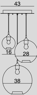
1209MX.3L SOSPENSIONE A PIASTRA / HANGING LAMP WITH CEILING PLATE Cable 150 cm 1 x E14 42 W 2 x E27 70 W
