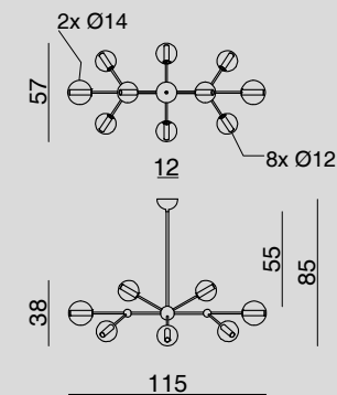
1574.10L.LIN LAMPADARIO / CHANDELIER Glass 10 x Ø 12-14 cm 10 x G9 33 W
