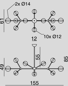
1574.12L.LIN LAMPADARIO / CHANDELIER Glass 12 x Ø 12-14 cm 12 x G9 33 W
