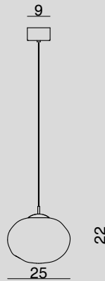
1643.1L SOSPENSIONE A ROSONE / HANGING LAMP WITH CANOPY Glass 1 x Ø 25 cm - Cable 200 cm 1 x LED 6 W DIMM
