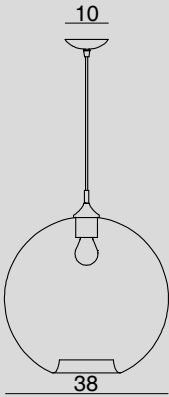
XXL1203.1L SOSPENSIONE A ROSONE / HANGING LAMP WITH CANOPY Glass 1 x Ø 38 cm - Cable 150 cm 1 x E27 70 W
